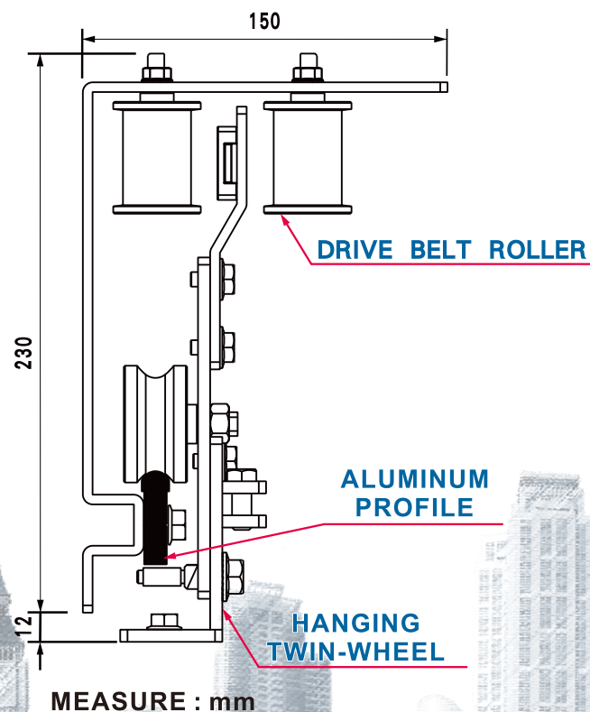
A. Position of drive belt roller (Near Belt-Roller)
