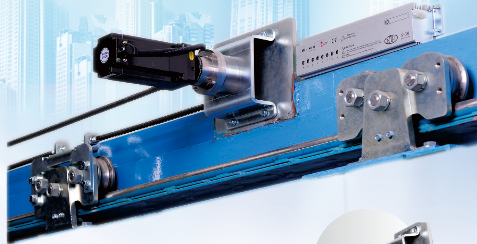
DC24V 250W BRUSHLESS DC MOTOR (PLANETARY GEAR)
