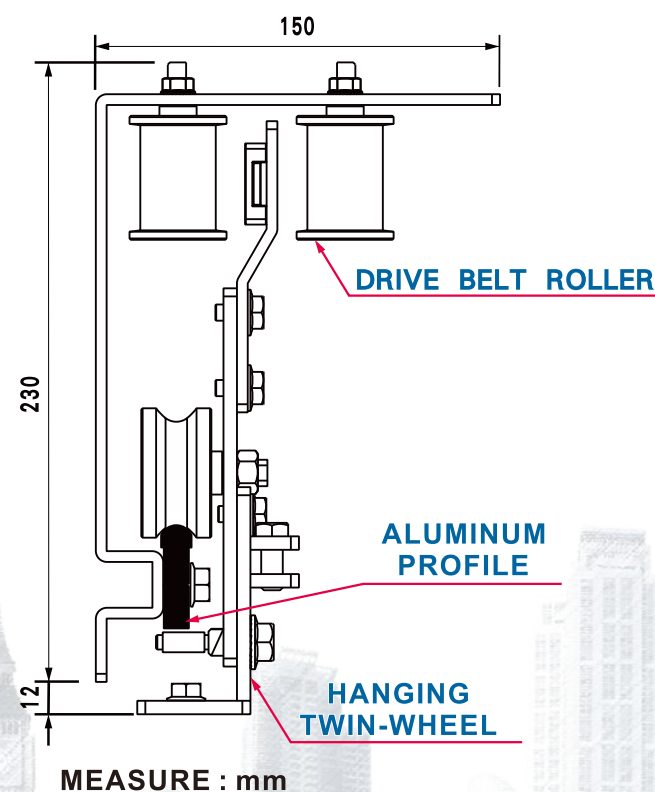
A. Position of drive belt roller (Near Belt-Roller) B. Position of drive belt roller (Near Motor)
