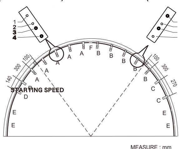
A. Position of drive belt roller (Near Belt-Roller) B. Position of drive belt roller (Near Motor)
