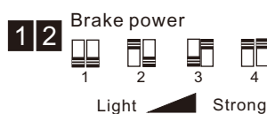
Fingered Switch
